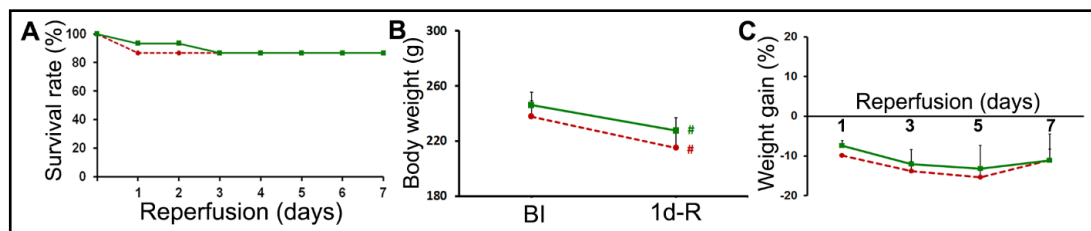
Fig. 3. Post-stroke mortality and body weight changes. Line graphs represent the percent survival rate (A), the reduction in body weight (B), or percent body weight gain (C) of rats. Dotted, and solid lines represent the data of ischemia-induced animals that were treated with vehicle, and exosomes respectively. BI-before ischemia; R-reperfusion. Error bars indicate SEM. n = 15 for mortality assessment and n = 7-9 for body weight assessments. # p < 0.05 vs. BI.
