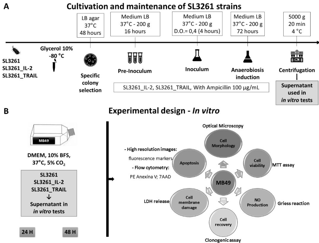
Supplementary Fig. 1. Schematic summary of established protocols. (A) Cultivation and maintenance of SL3261, SL3261_IL-2 and SL3261_TRAIL strains. (B) Techniques and in vitro tests with the MB49 cell line.
